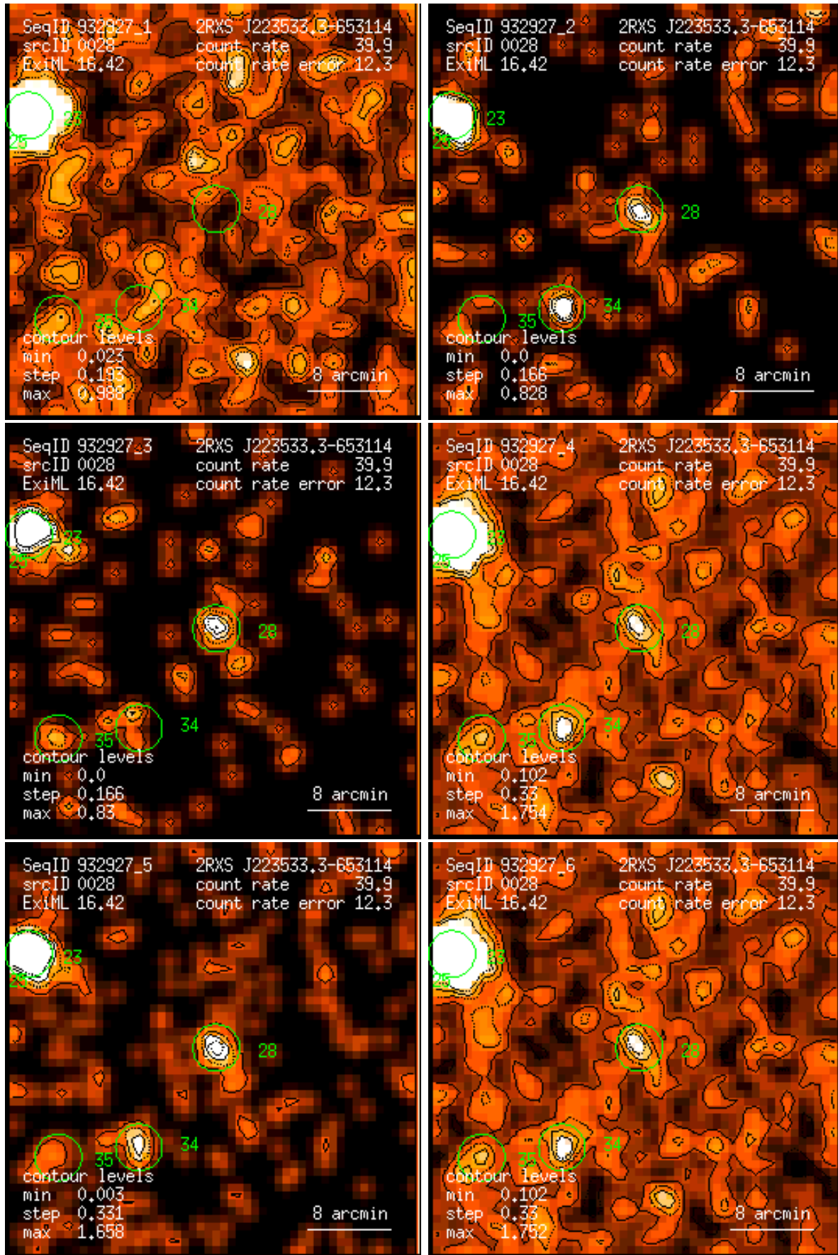
Figure 28: RASS 932927: detection 0028: band rate images, Gaussian filter: (1) PSPC channels 11 – 41, (2) 52 – 90, (3) 91 – 201, (4) 11 – 235, (5) 52 – 201, (6) 11 – 201. Broad band rates in counts/ks. Band rate contour levels in counts/ks/arcmin 2 .
