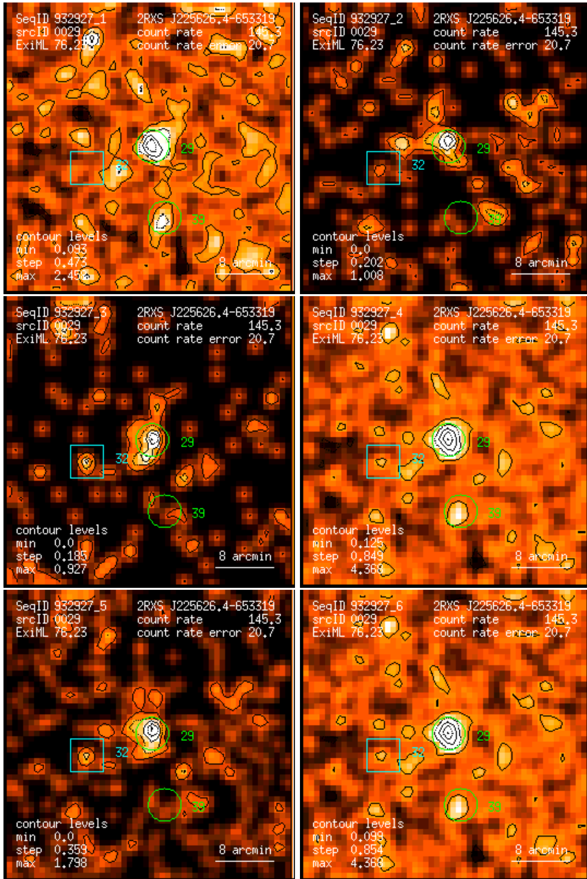
Figure 29: RASS 932927: detection 0029: band rate images, Gaussian filter: (1) PSPC channels 11 – 41, (2) 52 – 90, (3) 91 – 201, (4) 11 – 235, (5) 52 – 201, (6) 11 – 201. Broad band rates in counts/ks. Band rate contour levels in counts/ks/arcmin 2 .
