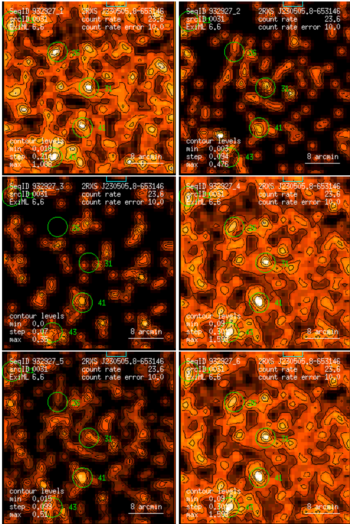
Figure 31: RASS 932927: detection 0031: band rate images, Gaussian filter: (1) PSPC channels 11 – 41, (2) 52 – 90, (3) 91 – 201, (4) 11 – 235, (5) 52 – 201, (6) 11 – 201. Broad band rates in counts/ks. Band rate contour levels in counts/ks/arcmin 2 .
