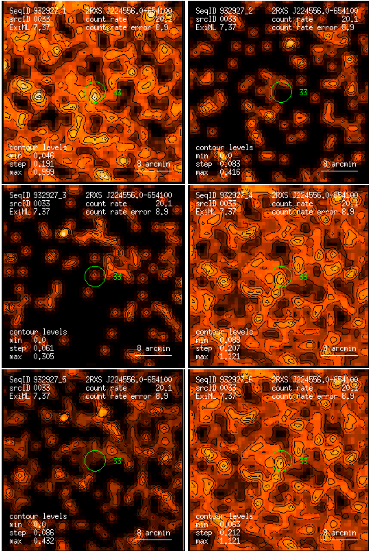
Figure 33: RASS 932927: detection 0033: band rate images, Gaussian filter: (1) PSPC channels 11 – 41, (2) 52 – 90, (3) 91 – 201, (4) 11 – 235, (5) 52 – 201, (6) 11 – 201. Broad band rates in counts/ks. Band rate contour levels in counts/ks/arcmin 2 .
