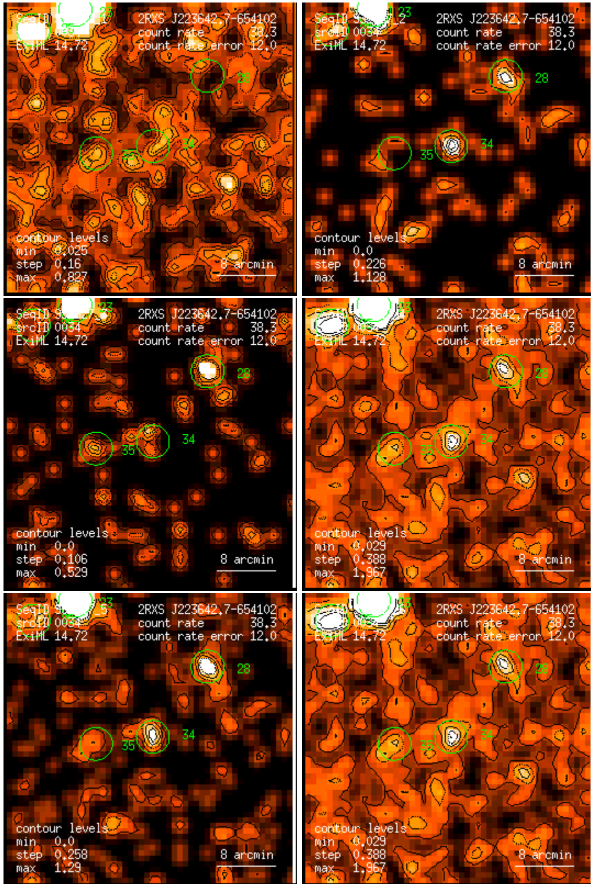
Figure 34: RASS 932927: detection 0034: band rate images, Gaussian filter: (1) PSPC channels 11 – 41, (2) 52 – 90, (3) 91 – 201, (4) 11 – 235, (5) 52 – 201, (6) 11 – 201. Broad band rates in counts/ks. Band rate contour levels in counts/ks/arcmin 2 .
