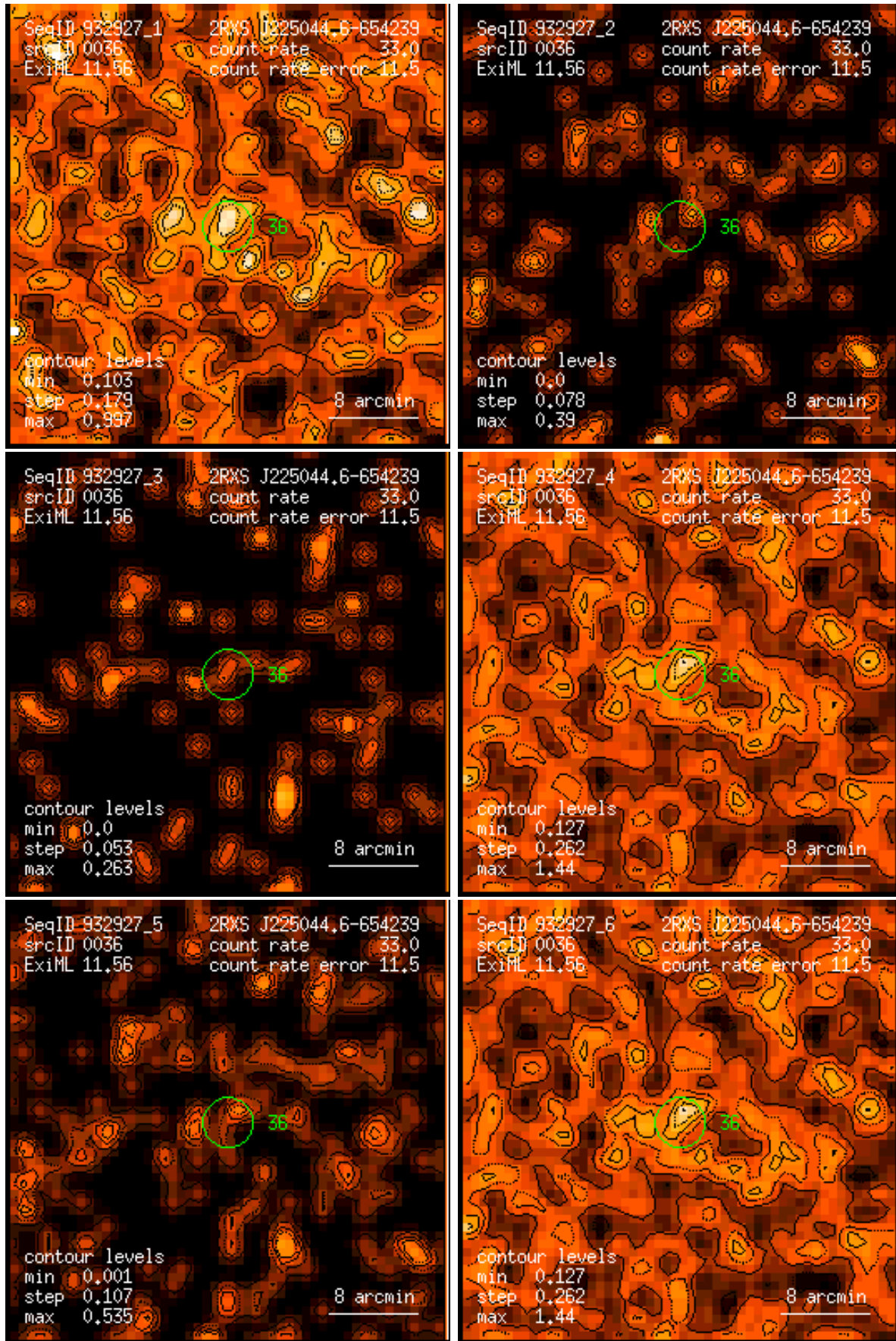
Figure 36: RASS 932927: detection 0036: band rate images, Gaussian filter: (1) PSPC channels 11 – 41, (2) 52 – 90, (3) 91 – 201, (4) 11 – 235, (5) 52 – 201, (6) 11 – 201. Broad band rates in counts/ks. Band rate contour levels in counts/ks/arcmin 2 .
