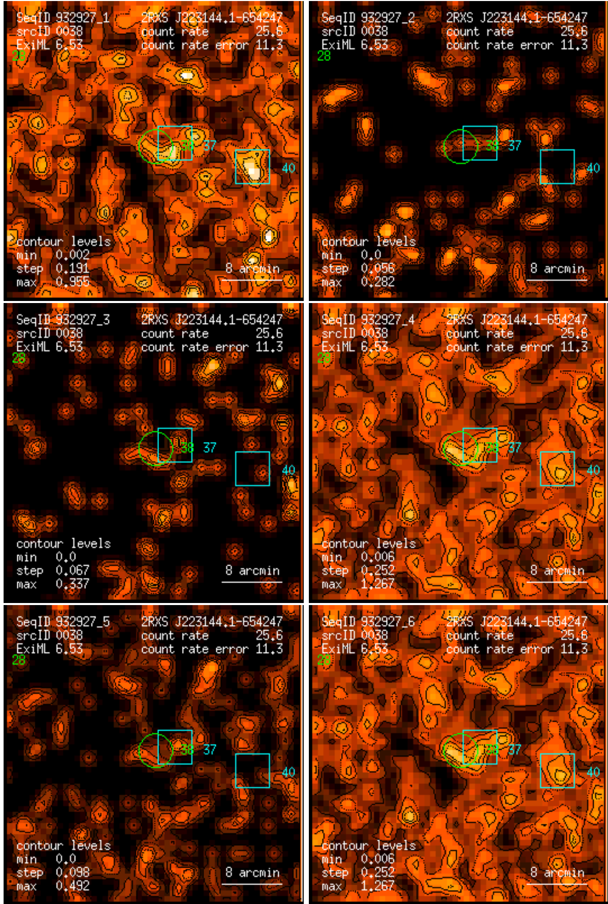
Figure 38: RASS 932927: detection 0038: band rate images, Gaussian filter: (1) PSPC channels 11 – 41, (2) 52 – 90, (3) 91 – 201, (4) 11 – 235, (5) 52 – 201, (6) 11 – 201. Broad band rates in counts/ks. Band rate contour levels in counts/ks/arcmin 2 .
