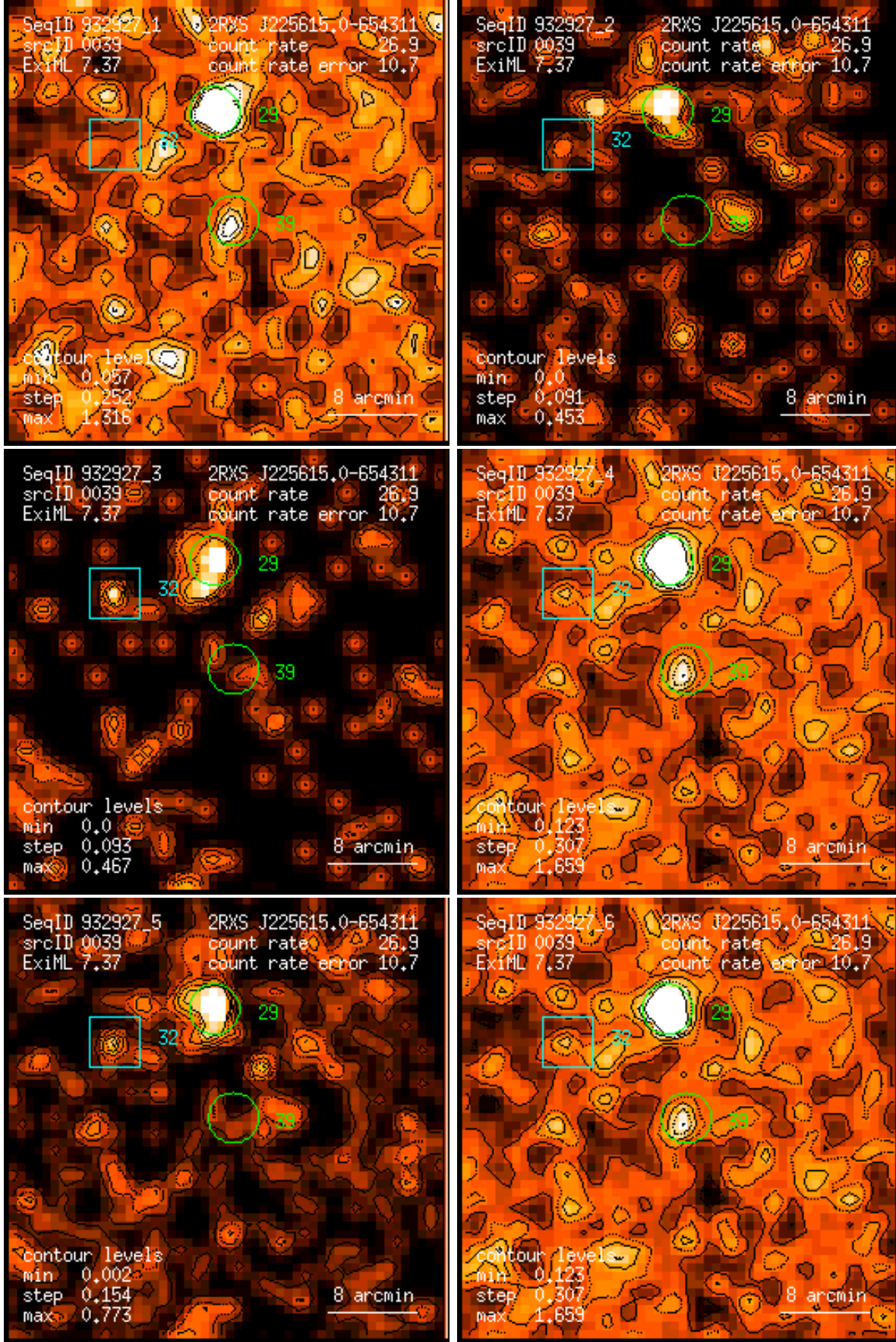
Figure 39: RASS 932927: detection 0039: band rate images, Gaussian filter: (1) PSPC channels 11 – 41, (2) 52 – 90, (3) 91 – 201, (4) 11 – 235, (5) 52 – 201, (6) 11 – 201. Broad band rates in counts/ks. Band rate contour levels in counts/ks/arcmin 2 .
