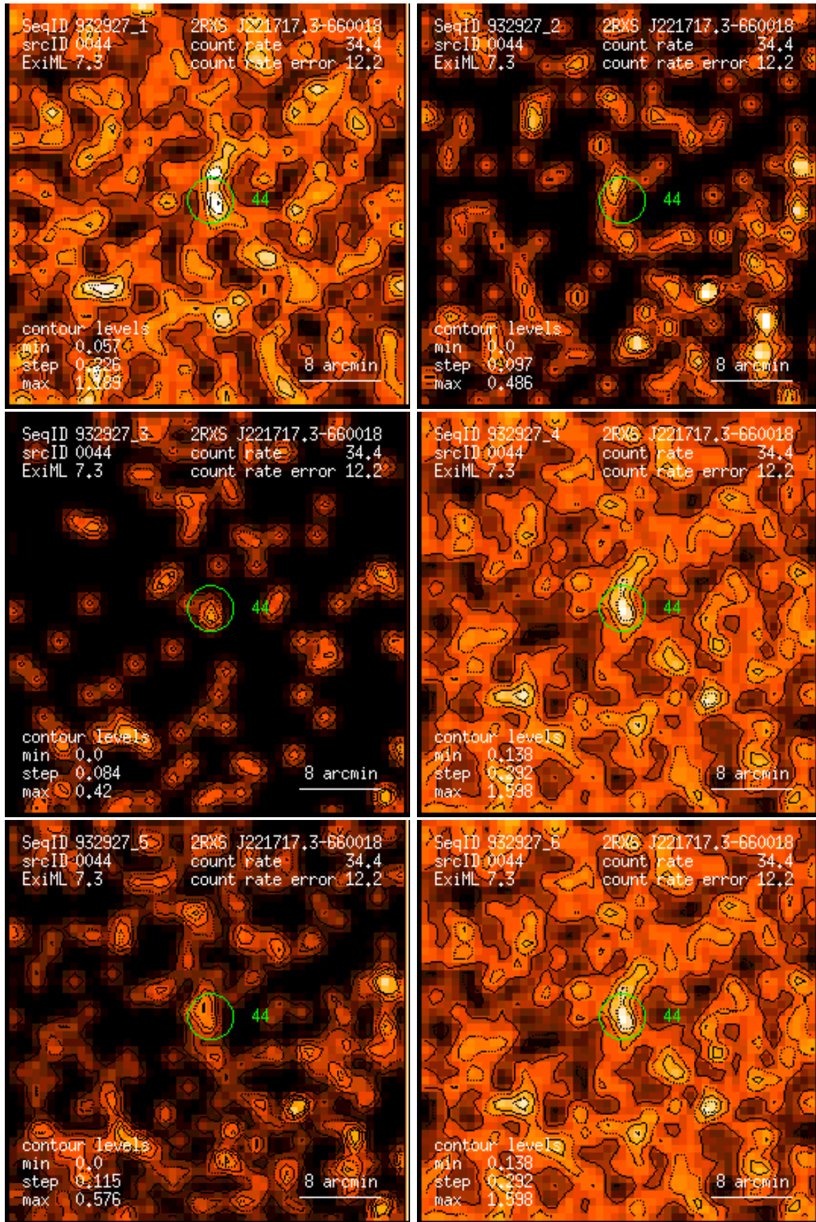
Figure 44: RASS 932927: detection 0044: band rate images, Gaussian filter: (1) PSPC channels 11 – 41, (2) 52 – 90, (3) 91 – 201, (4) 11 – 235, (5) 52 – 201, (6) 11 – 201. Broad band rates in counts/ks. Band rate contour levels in counts/ks/arcmin 2 .
