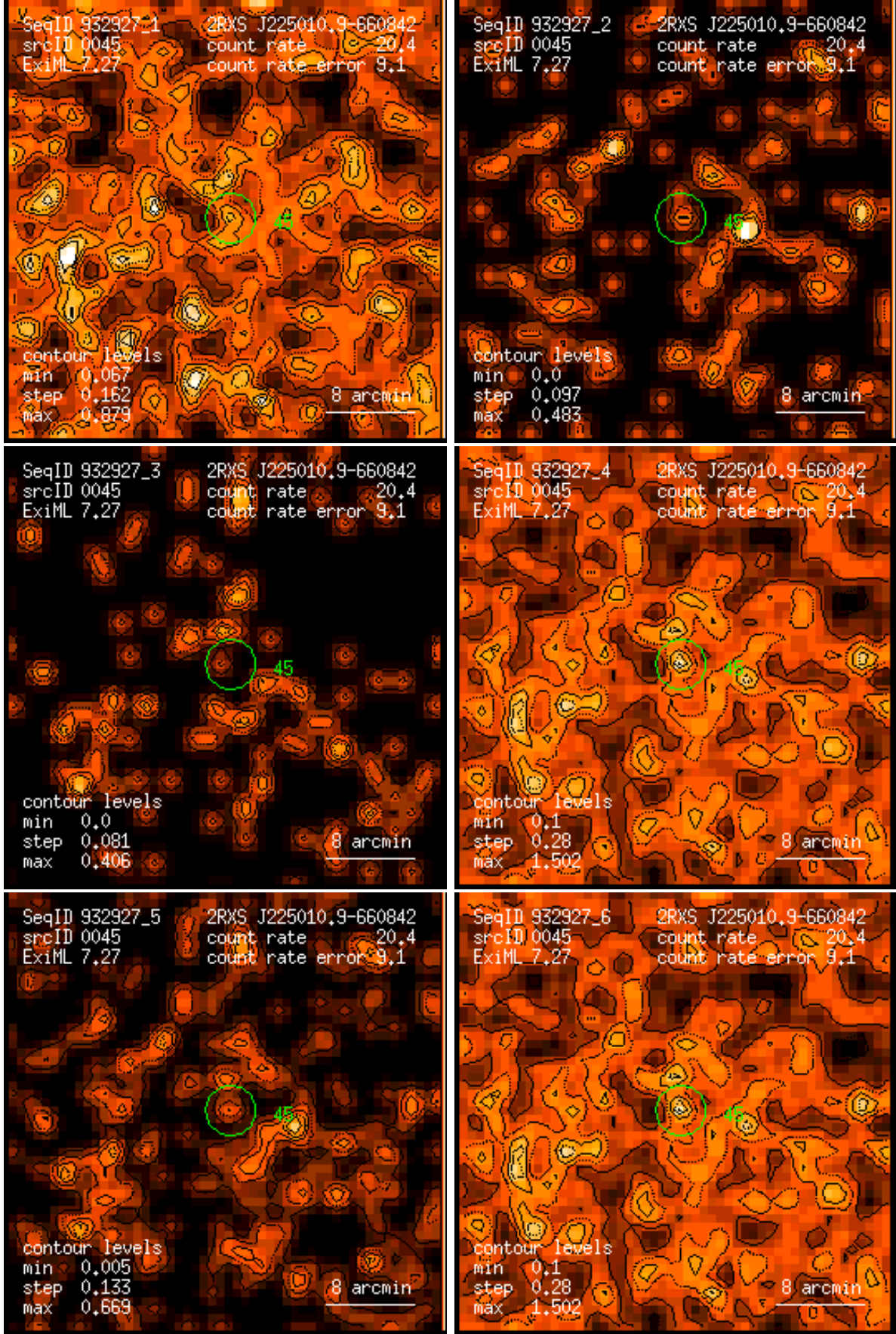
Figure 45: RASS 932927: detection 0045: band rate images, Gaussian filter: (1) PSPC channels 11 – 41, (2) 52 – 90, (3) 91 – 201, (4) 11 – 235, (5) 52 – 201, (6) 11 – 201. Broad band rates in counts/ks. Band rate contour levels in counts/ks/arcmin 2 .
