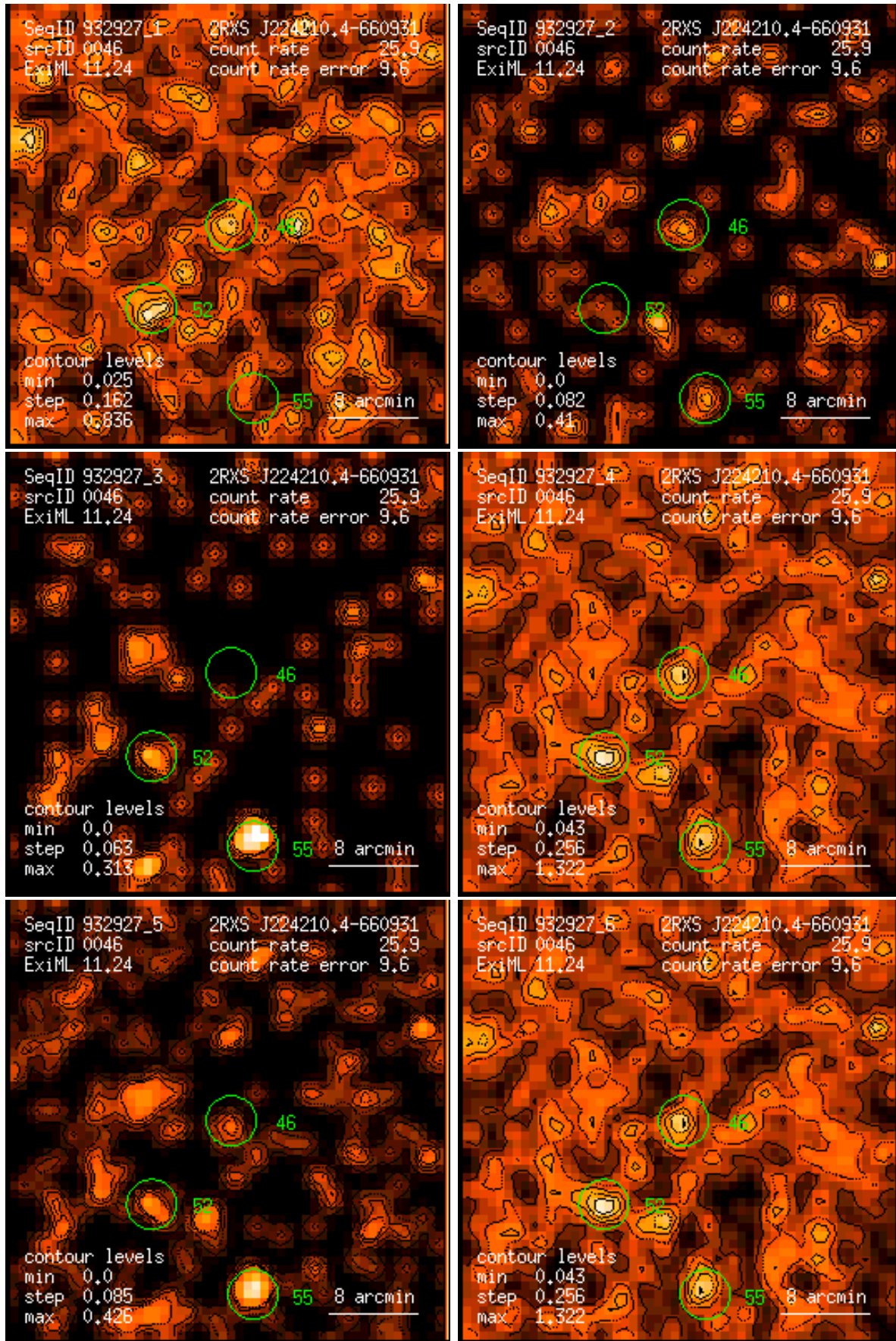
Figure 46: RASS 932927: detection 0046: band rate images, Gaussian filter: (1) PSPC channels 11 – 41, (2) 52 – 90, (3) 91 – 201, (4) 11 – 235, (5) 52 – 201, (6) 11 – 201. Broad band rates in counts/ks. Band rate contour levels in counts/ks/arcmin 2 .
