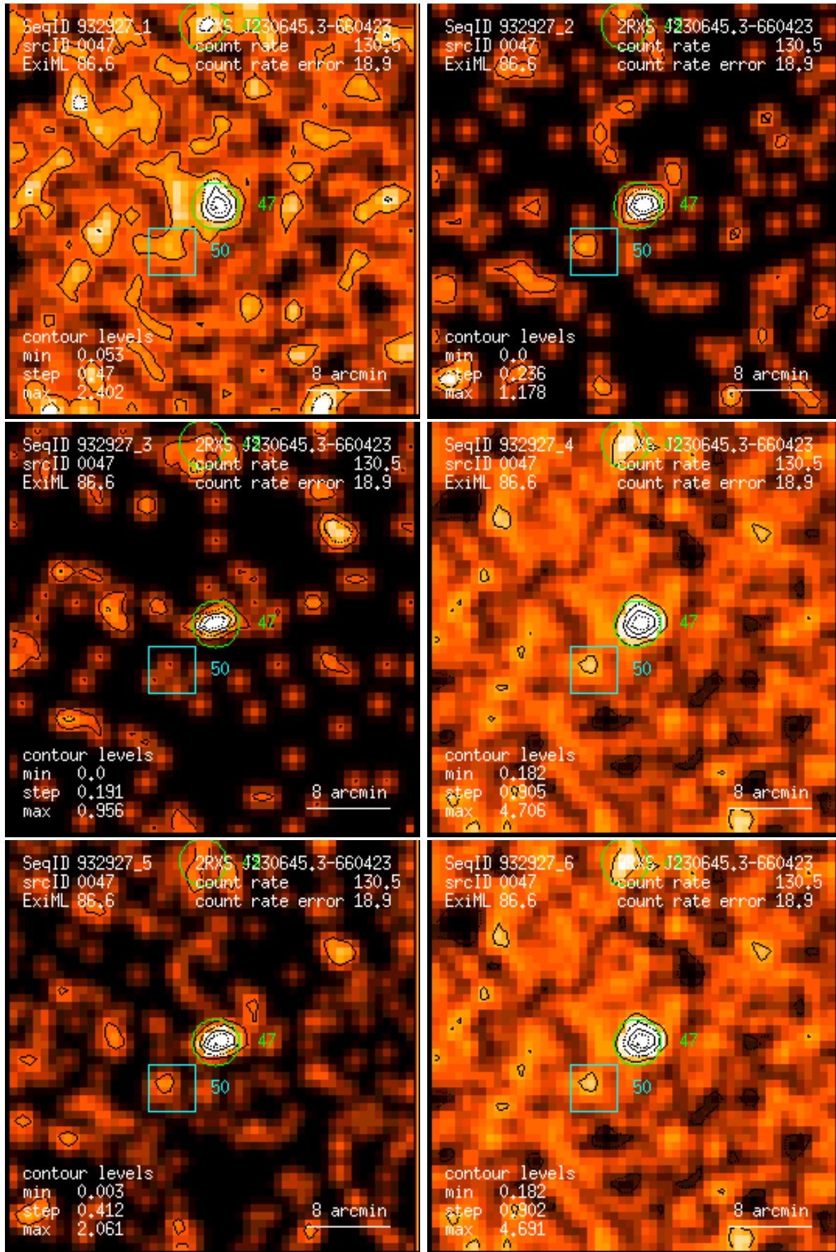
Figure 47: RASS 932927: detection 0047: band rate images, Gaussian filter: (1) PSPC channels 11 – 41, (2) 52 – 90, (3) 91 – 201, (4) 11 – 235, (5) 52 – 201, (6) 11 – 201. Broad band rates in counts/ks. Band rate contour levels in counts/ks/arcmin 2 .
