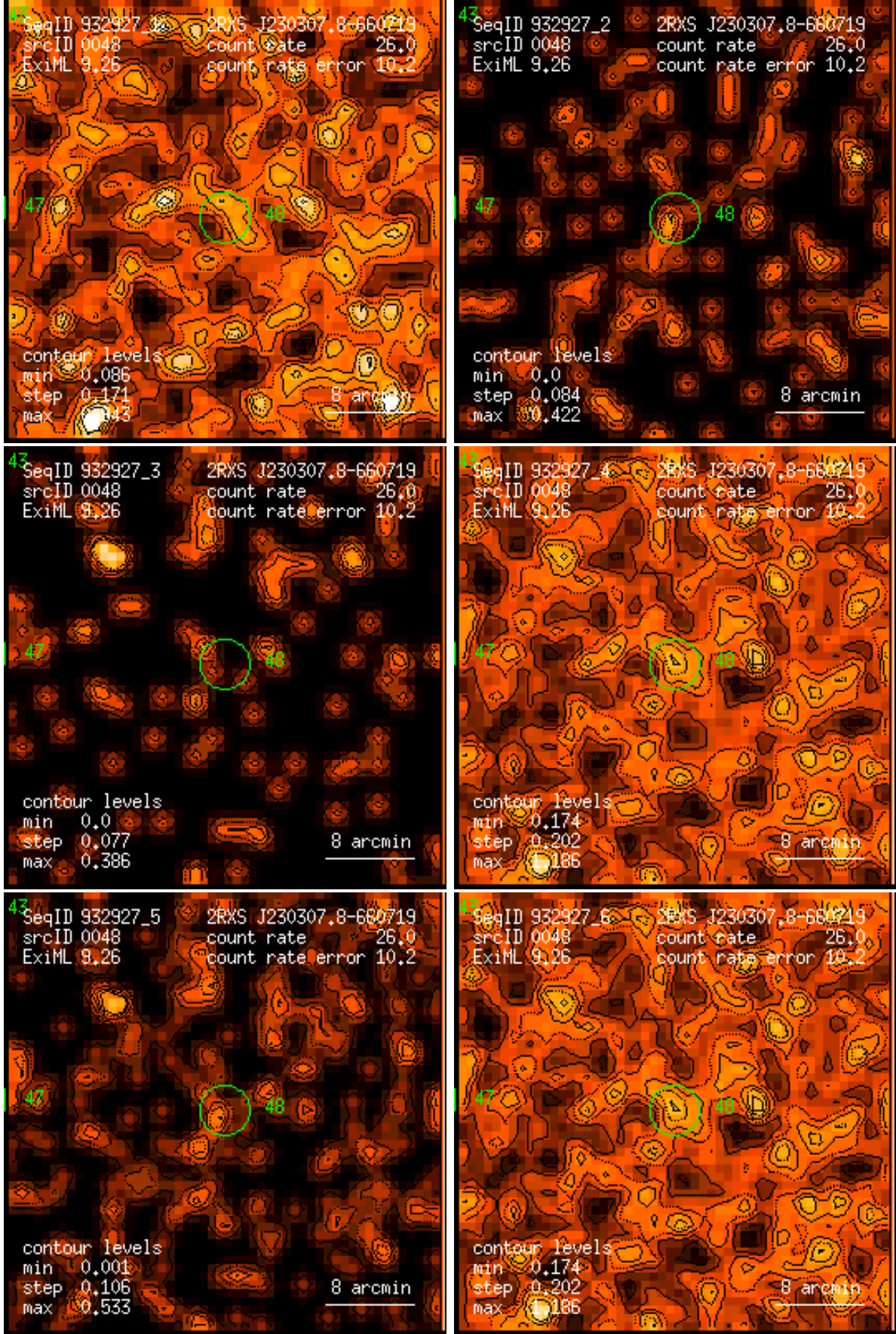
Figure 48: RASS 932927: detection 0048: band rate images, Gaussian filter: (1) PSPC channels 11 – 41, (2) 52 – 90, (3) 91 – 201, (4) 11 – 235, (5) 52 – 201, (6) 11 – 201. Broad band rates in counts/ks. Band rate contour levels in counts/ks/arcmin 2 .
