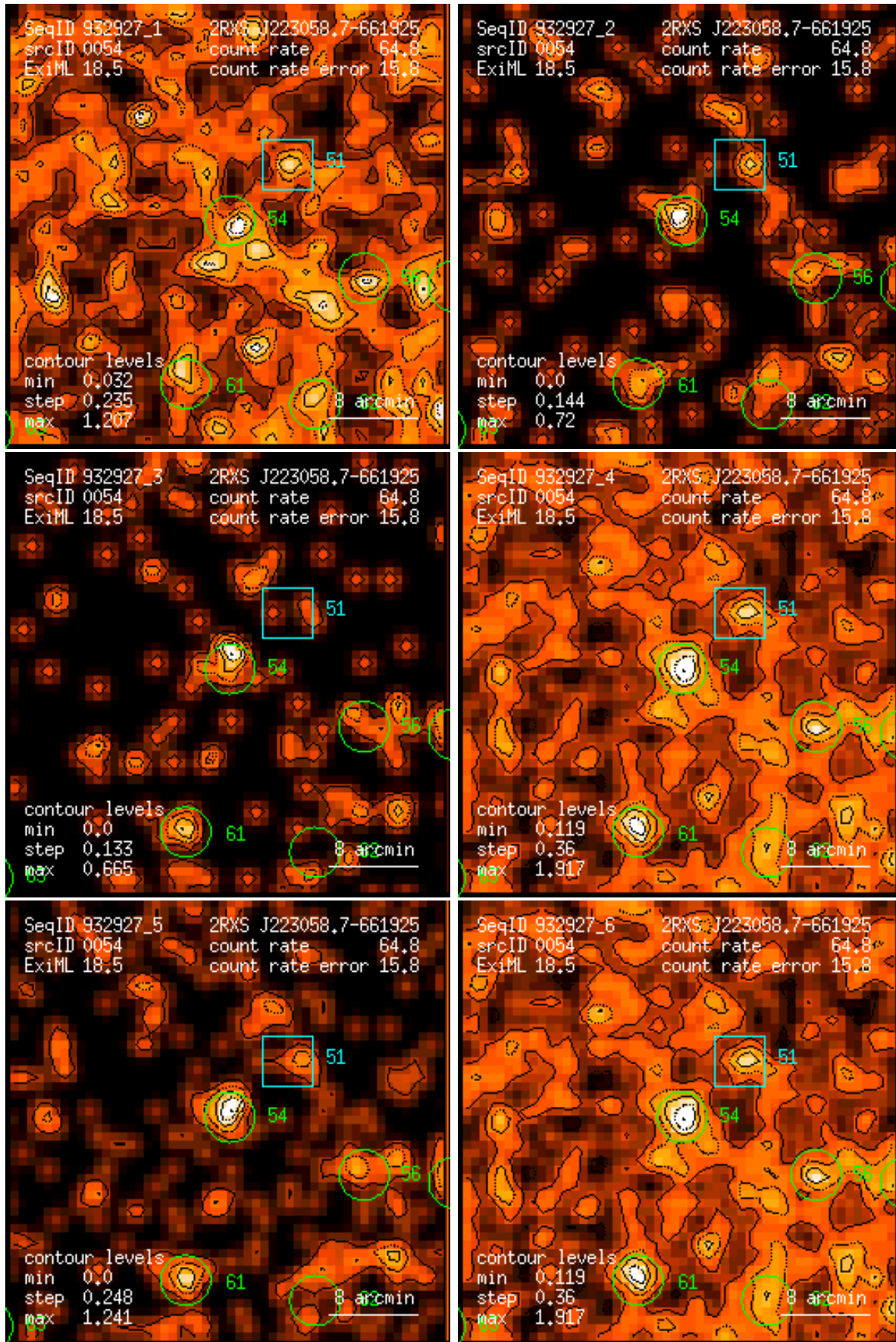
Figure 54: RASS 932927: detection 0054: band rate images, Gaussian filter: (1) PSPC channels 11 – 41, (2) 52 – 90, (3) 91 – 201, (4) 11 – 235, (5) 52 – 201, (6) 11 – 201. Broad band rates in counts/ks. Band rate contour levels in counts/ks/arcmin 2 .
