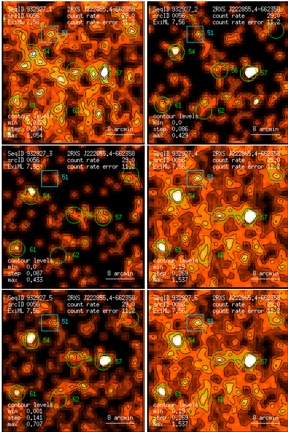
Figure 56: RASS 932927: detection 0056: band rate images, Gaussian filter: (1) PSPC channels 11 – 41, (2) 52 – 90, (3) 91 – 201, (4) 11 – 235, (5) 52 – 201, (6) 11 – 201. Broad band rates in counts/ks. Band rate contour levels in counts/ks/arcmin 2 .
