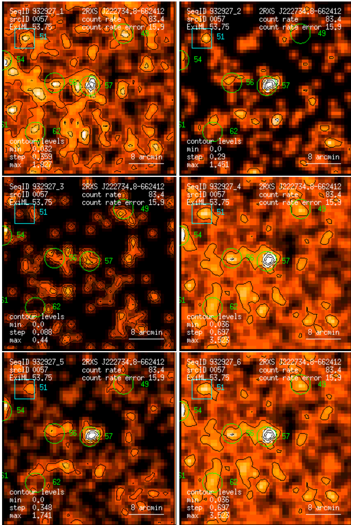
Figure 57: RASS 932927: detection 0057: band rate images, Gaussian filter: (1) PSPC channels 11 – 41, (2) 52 – 90, (3) 91 – 201, (4) 11 – 235, (5) 52 – 201, (6) 11 – 201. Broad band rates in counts/ks. Band rate contour levels in counts/ks/arcmin 2 .
