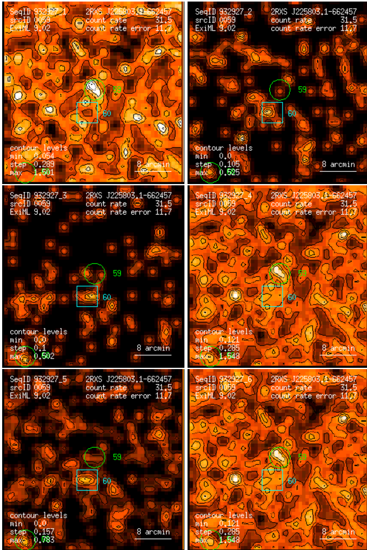
Figure 59: RASS 932927: detection 0059: band rate images, Gaussian filter: (1) PSPC channels 11 – 41, (2) 52 – 90, (3) 91 – 201, (4) 11 – 235, (5) 52 – 201, (6) 11 – 201. Broad band rates in counts/ks. Band rate contour levels in counts/ks/arcmin 2 .
