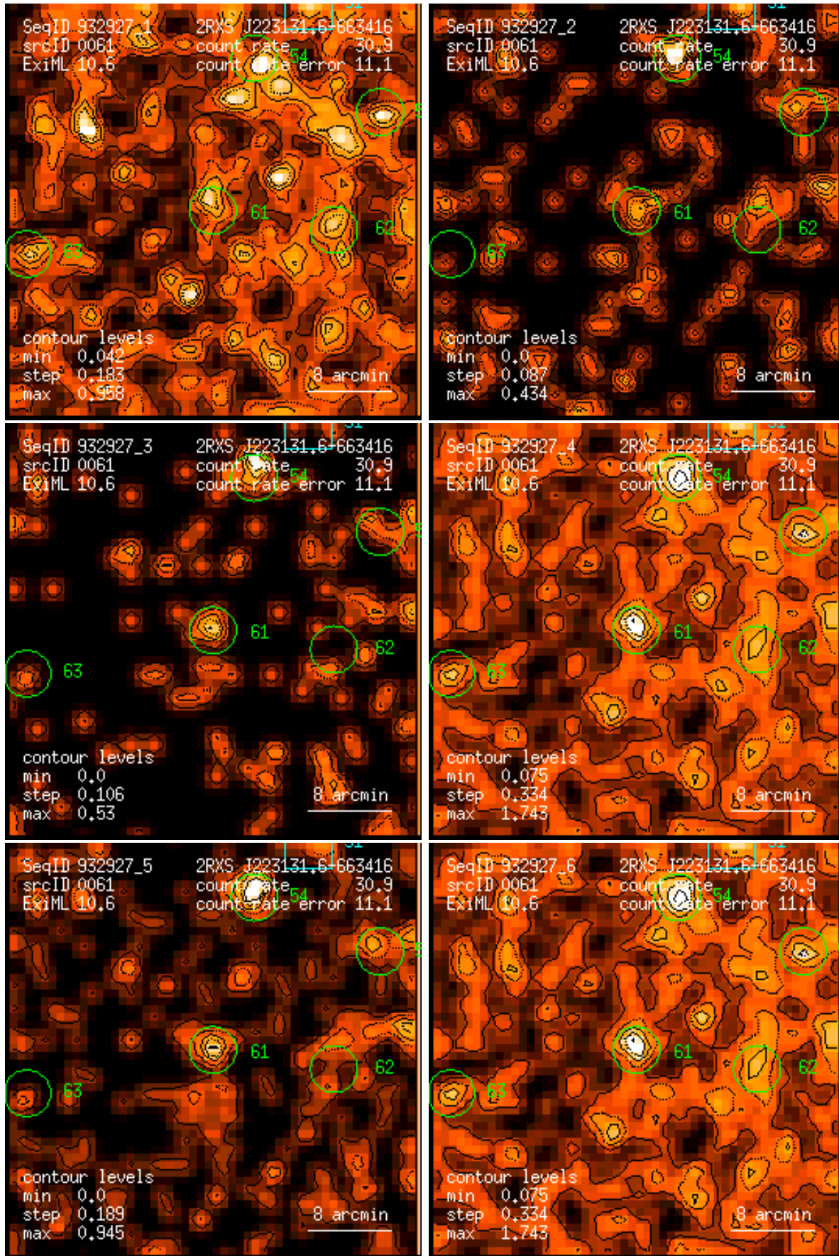
Figure 61: RASS 932927: detection 0061: band rate images, Gaussian filter: (1) PSPC channels 11 – 41, (2) 52 – 90, (3) 91 – 201, (4) 11 – 235, (5) 52 – 201, (6) 11 – 201. Broad band rates in counts/ks. Band rate contour levels in counts/ks/arcmin 2 .
