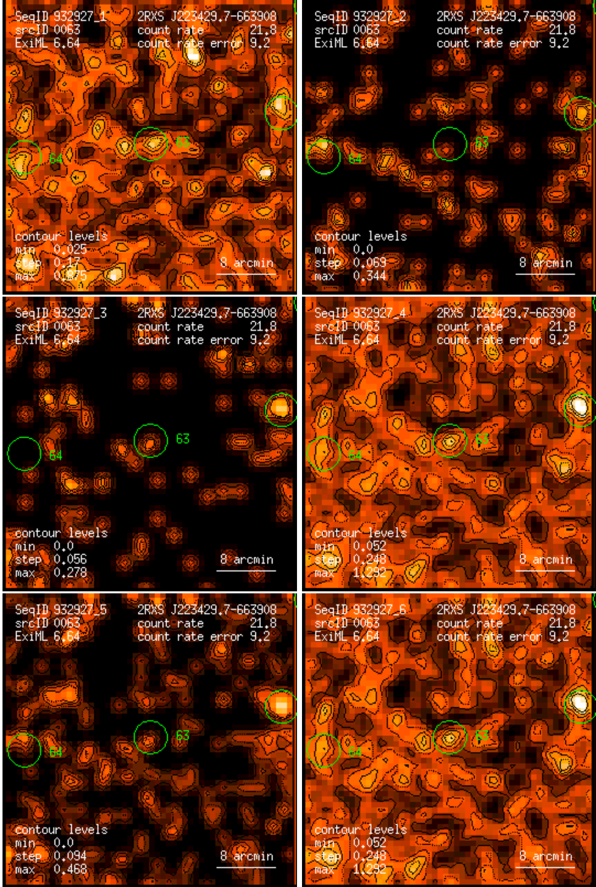
Figure 63: RASS 932927: detection 0063: band rate images, Gaussian filter: (1) PSPC channels 11 – 41, (2) 52 – 90, (3) 91 – 201, (4) 11 – 235, (5) 52 – 201, (6) 11 – 201. Broad band rates in counts/ks. Band rate contour levels in counts/ks/arcmin 2 .
