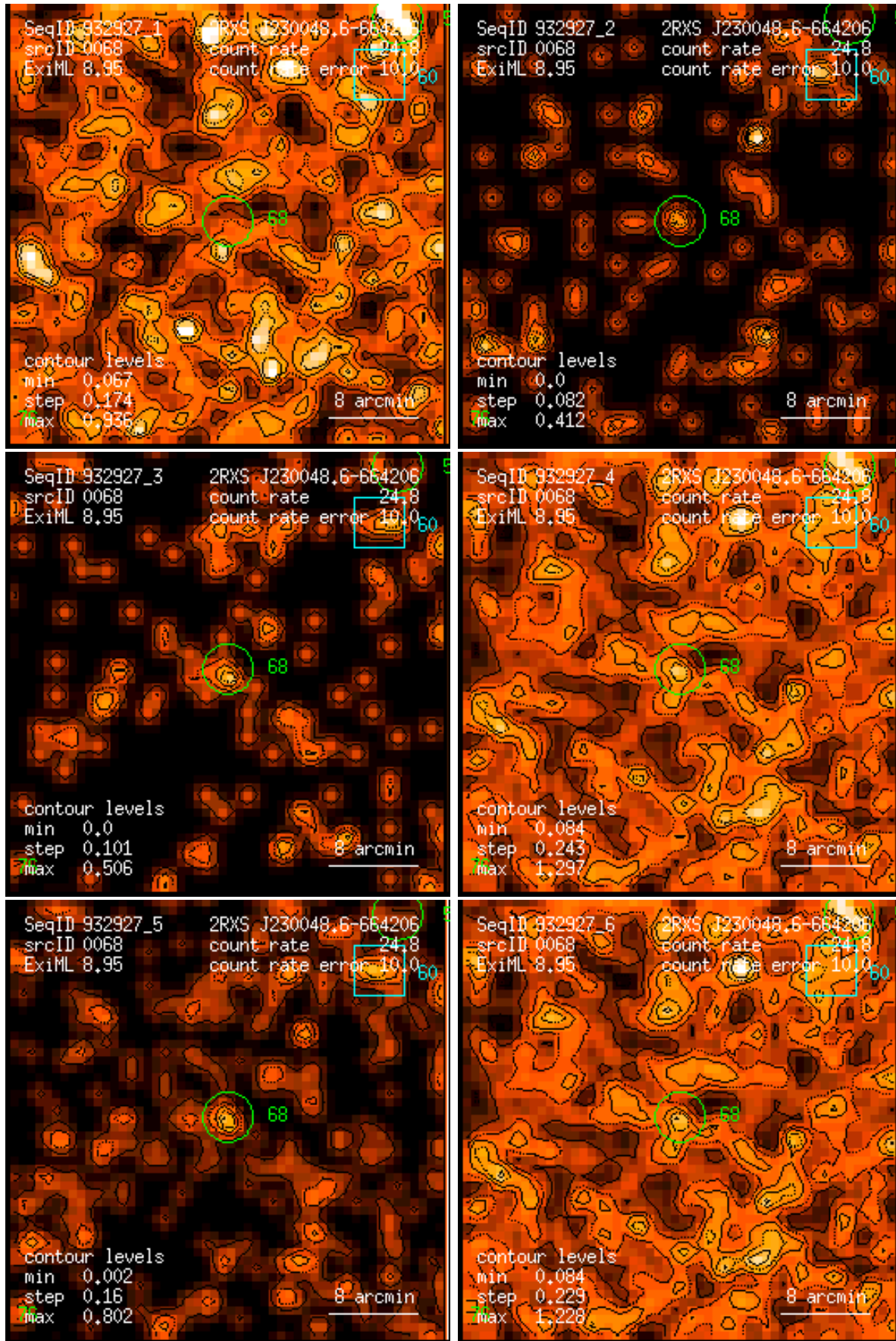
Figure 68: RASS 932927: detection 0068: band rate images, Gaussian filter: (1) PSPC channels 11 – 41, (2) 52 – 90, (3) 91 – 201, (4) 11 – 235, (5) 52 – 201, (6) 11 – 201. Broad band rates in counts/ks. Band rate contour levels in counts/ks/arcmin 2 .
