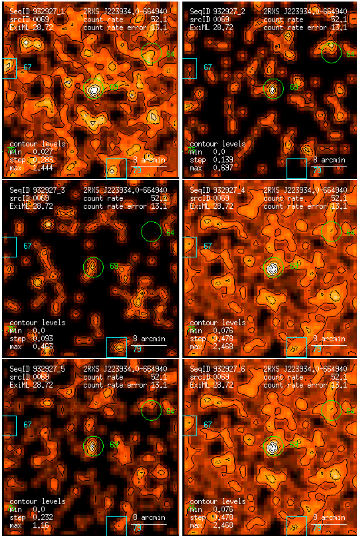
Figure 69: RASS 932927: detection 0069: band rate images, Gaussian filter: (1) PSPC channels 11 – 41, (2) 52 – 90, (3) 91 – 201, (4) 11 – 235, (5) 52 – 201, (6) 11 – 201. Broad band rates in counts/ks. Band rate contour levels in counts/ks/arcmin 2 .
