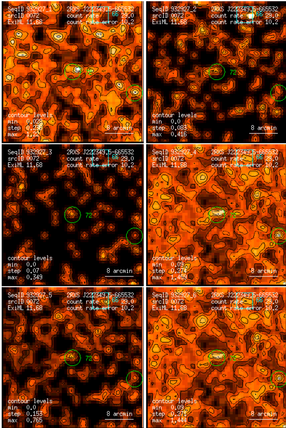
Figure 72: RASS 932927: detection 0072: band rate images, Gaussian filter: (1) PSPC channels 11 – 41, (2) 52 – 90, (3) 91 – 201, (4) 11 – 235, (5) 52 – 201, (6) 11 – 201. Broad band rates in counts/ks. Band rate contour levels in counts/ks/arcmin 2 .
