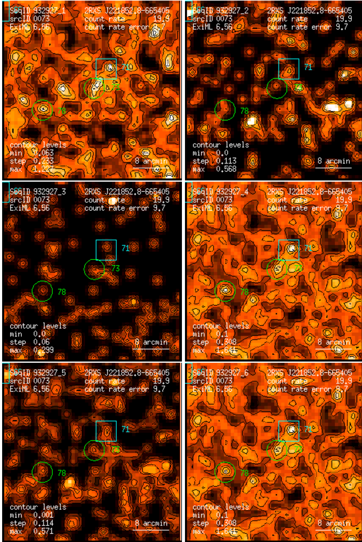
Figure 73: RASS 932927: detection 0073: band rate images, Gaussian filter: (1) PSPC channels 11 – 41, (2) 52 – 90, (3) 91 – 201, (4) 11 – 235, (5) 52 – 201, (6) 11 – 201. Broad band rates in counts/ks. Band rate contour levels in counts/ks/arcmin 2 .
