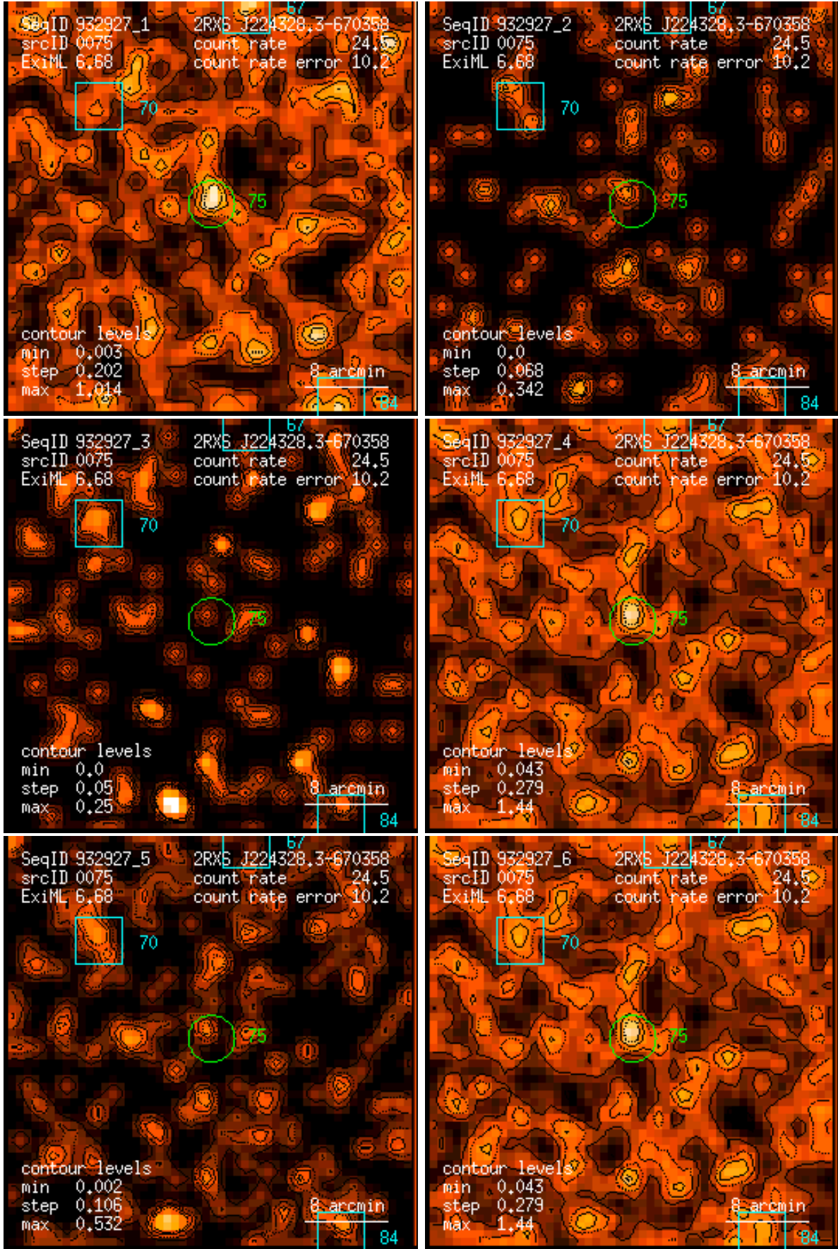
Figure 75: RASS 932927: detection 0075: band rate images, Gaussian filter: (1) PSPC channels 11 – 41, (2) 52 – 90, (3) 91 – 201, (4) 11 – 235, (5) 52 – 201, (6) 11 – 201. Broad band rates in counts/ks. Band rate contour levels in counts/ks/arcmin 2 .
