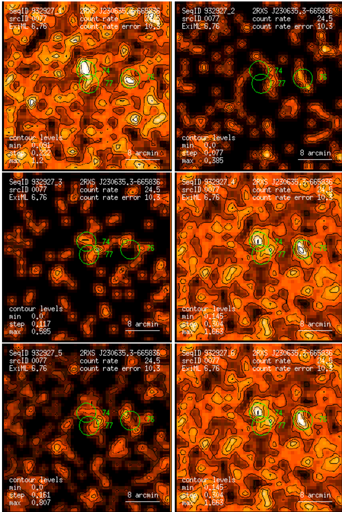
Figure 77: RASS 932927: detection 0077: band rate images, Gaussian filter: (1) PSPC channels 11 – 41, (2) 52 – 90, (3) 91 – 201, (4) 11 – 235, (5) 52 – 201, (6) 11 – 201. Broad band rates in counts/ks. Band rate contour levels in counts/ks/arcmin 2 .
