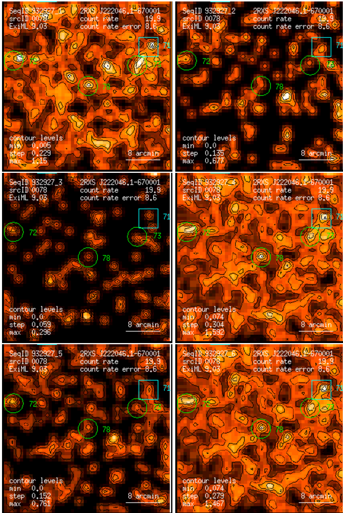
Figure 78: RASS 932927: detection 0078: band rate images, Gaussian filter: (1) PSPC channels 11 – 41, (2) 52 – 90, (3) 91 – 201, (4) 11 – 235, (5) 52 – 201, (6) 11 – 201. Broad band rates in counts/ks. Band rate contour levels in counts/ks/arcmin 2 .
