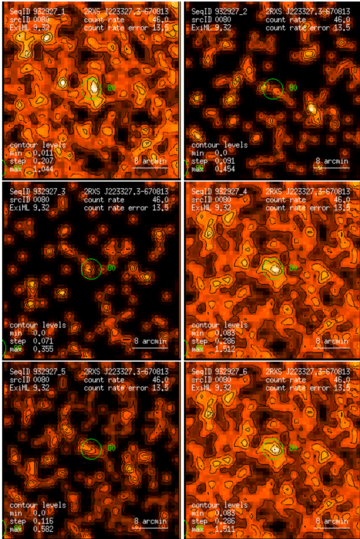
Figure 80: RASS 932927: detection 0080: band rate images, Gaussian filter: (1) PSPC channels 11 – 41, (2) 52 – 90, (3) 91 – 201, (4) 11 – 235, (5) 52 – 201, (6) 11 – 201. Broad band rates in counts/ks. Band rate contour levels in counts/ks/arcmin 2 .
