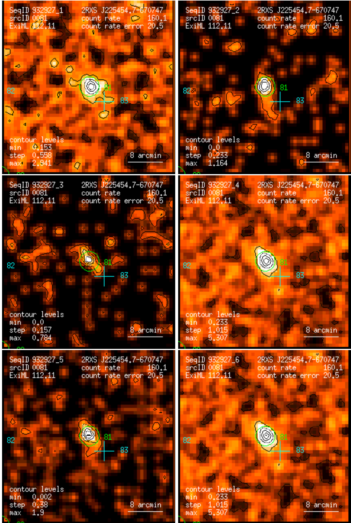
Figure 81: RASS 932927: detection 0081: band rate images, Gaussian filter: (1) PSPC channels 11 – 41, (2) 52 – 90, (3) 91 – 201, (4) 11 – 235, (5) 52 – 201, (6) 11 – 201. Broad band rates in counts/ks. Band rate contour levels in counts/ks/arcmin 2 .
