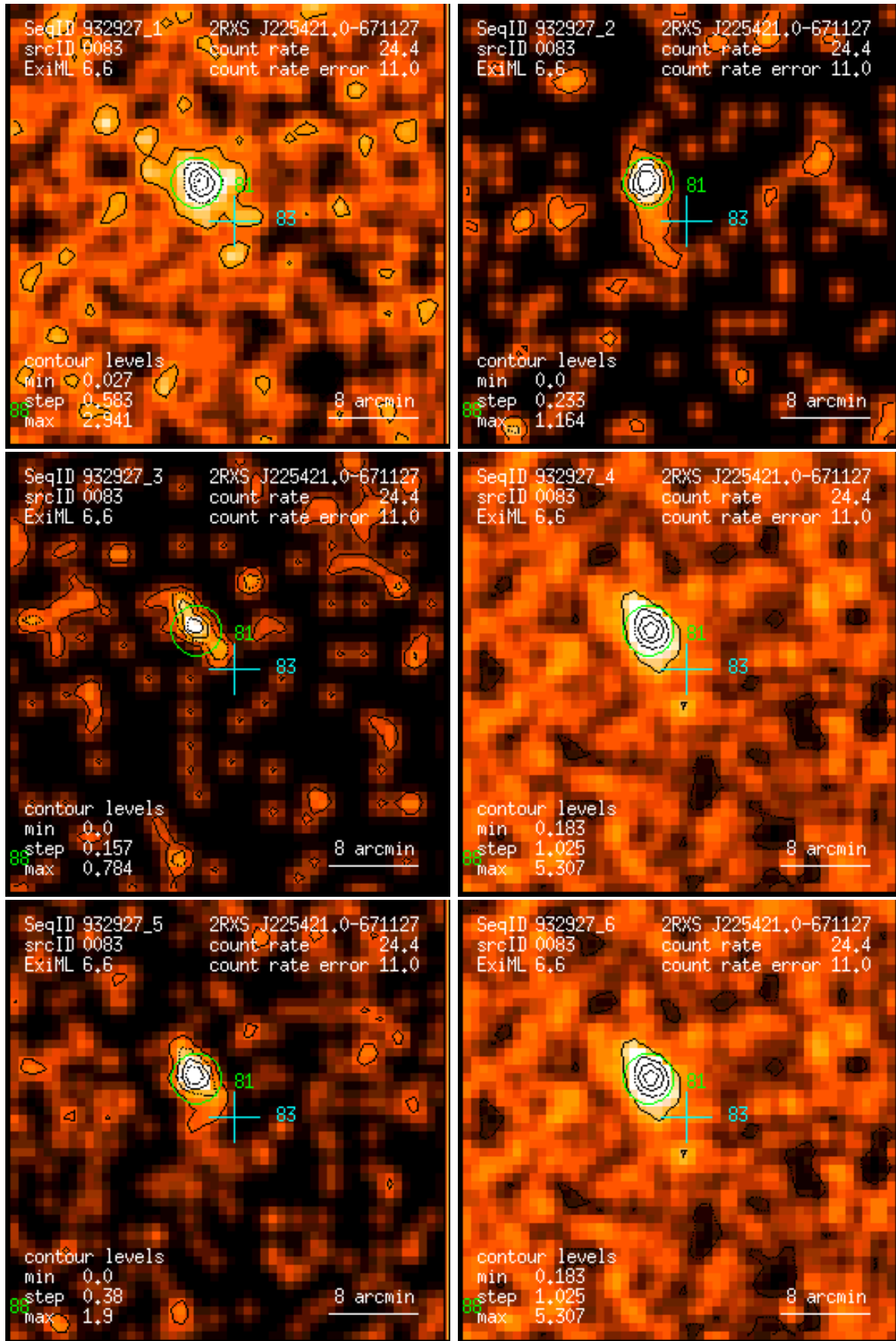
Figure 83: RASS 932927: detection 0083: band rate images, Gaussian filter: (1) PSPC channels 11 – 41, (2) 52 – 90, (3) 91 – 201, (4) 11 – 235, (5) 52 – 201, (6) 11 – 201. Broad band rates in counts/ks. Band rate contour levels in counts/ks/arcmin 2 .
