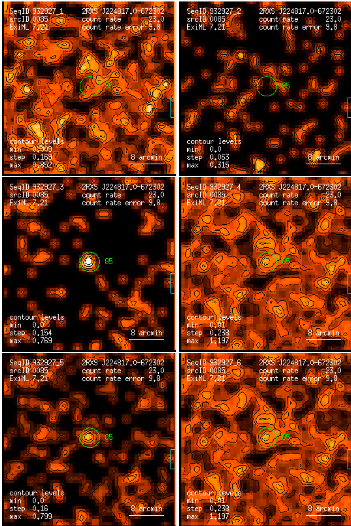
Figure 85: RASS 932927: detection 0085: band rate images, Gaussian filter: (1) PSPC channels 11 – 41, (2) 52 – 90, (3) 91 – 201, (4) 11 – 235, (5) 52 – 201, (6) 11 – 201. Broad band rates in counts/ks. Band rate contour levels in counts/ks/arcmin 2 .
