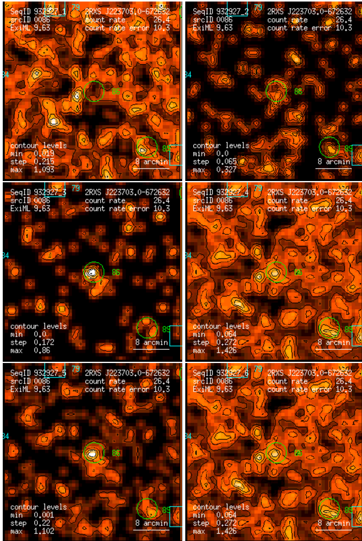
Figure 86: RASS 932927: detection 0086: band rate images, Gaussian filter: (1) PSPC channels 11 – 41, (2) 52 – 90, (3) 91 – 201, (4) 11 – 235, (5) 52 – 201, (6) 11 – 201. Broad band rates in counts/ks. Band rate contour levels in counts/ks/arcmin 2 .
