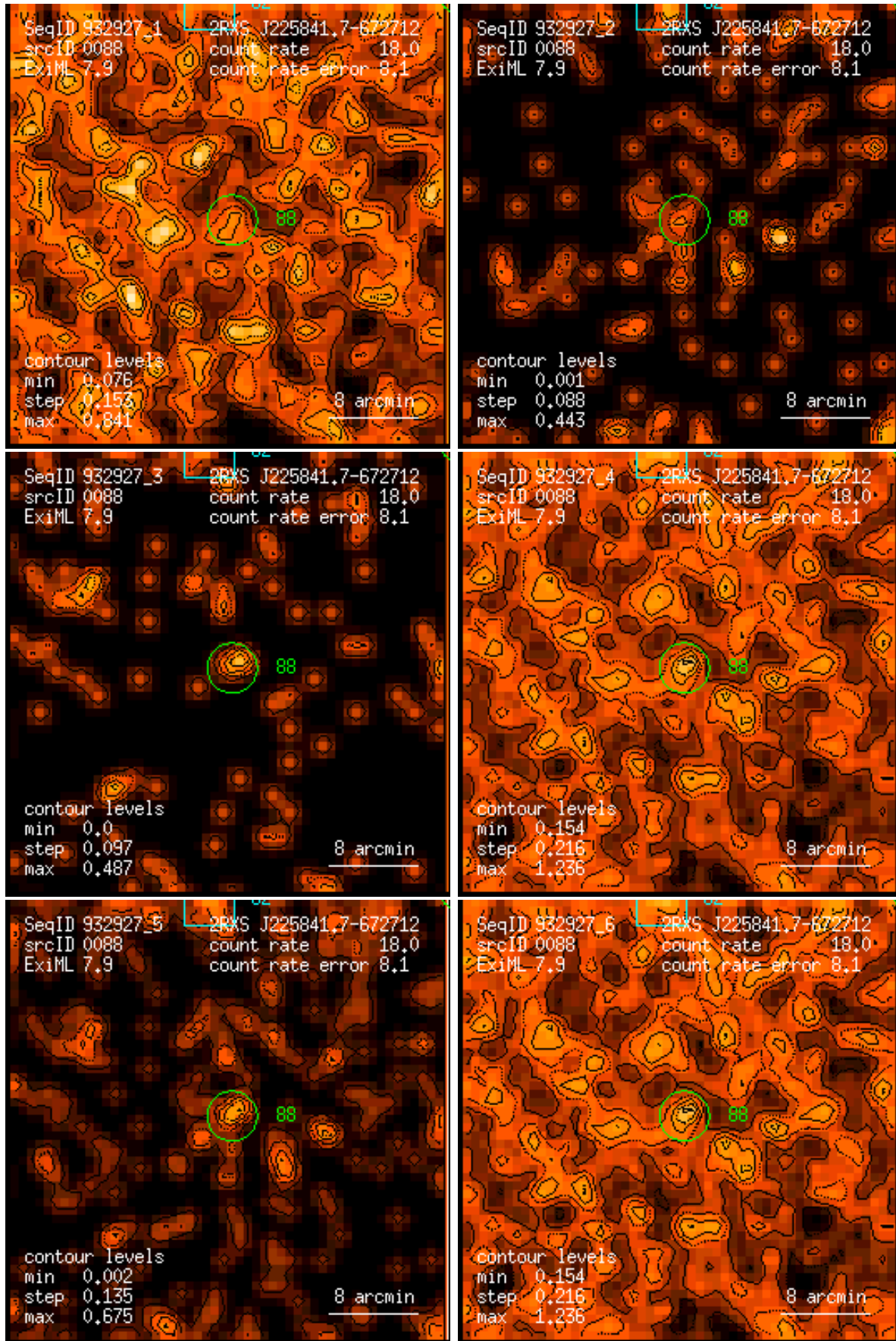
Figure 88: RASS 932927: detection 0088: band rate images, Gaussian filter: (1) PSPC channels 11 – 41, (2) 52 – 90, (3) 91 – 201, (4) 11 – 235, (5) 52 – 201, (6) 11 – 201. Broad band rates in counts/ks. Band rate contour levels in counts/ks/arcmin 2 .
