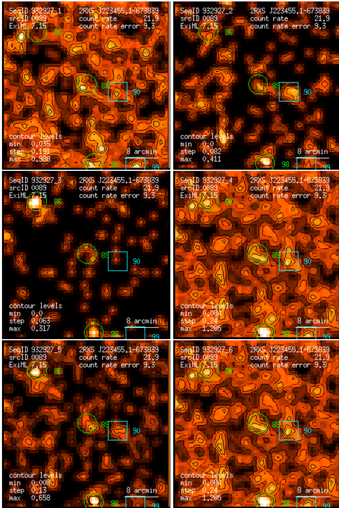
Figure 89: RASS 932927: detection 0089: band rate images, Gaussian filter: (1) PSPC channels 11 – 41, (2) 52 – 90, (3) 91 – 201, (4) 11 – 235, (5) 52 – 201, (6) 11 – 201. Broad band rates in counts/ks. Band rate contour levels in counts/ks/arcmin 2 .
