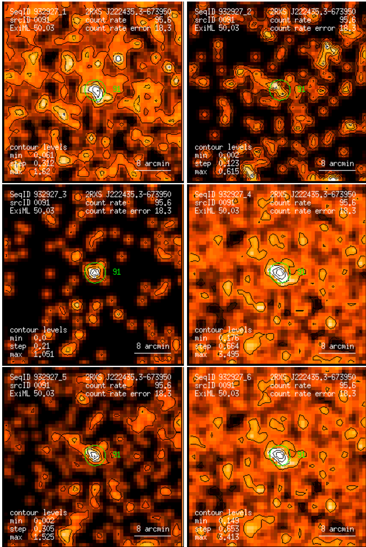
Figure 91: RASS 932927: detection 0091: band rate images, Gaussian filter: (1) PSPC channels 11 – 41, (2) 52 – 90, (3) 91 – 201, (4) 11 – 235, (5) 52 – 201, (6) 11 – 201. Broad band rates in counts/ks. Band rate contour levels in counts/ks/arcmin 2 .
