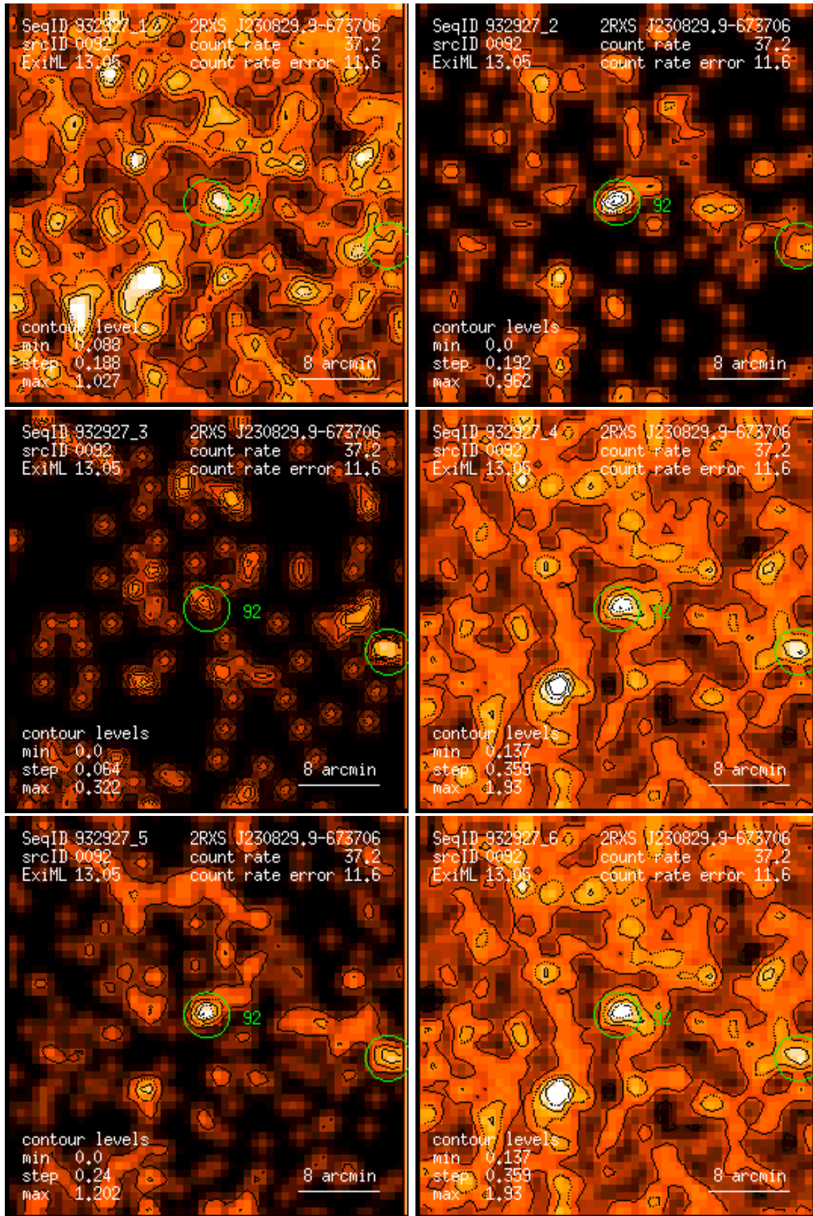
Figure 92: RASS 932927: detection 0092: band rate images, Gaussian filter: (1) PSPC channels 11 – 41, (2) 52 – 90, (3) 91 – 201, (4) 11 – 235, (5) 52 – 201, (6) 11 – 201. Broad band rates in counts/ks. Band rate contour levels in counts/ks/arcmin 2 .
