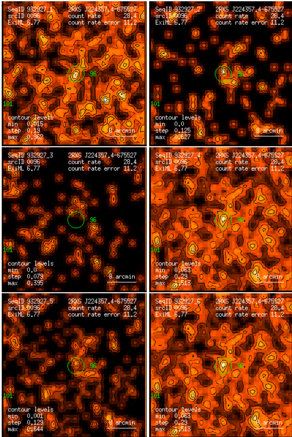
Figure 96: RASS 932927: detection 0096: band rate images, Gaussian filter: (1) PSPC channels 11 – 41, (2) 52 – 90, (3) 91 – 201, (4) 11 – 235, (5) 52 – 201, (6) 11 – 201. Broad band rates in counts/ks. Band rate contour levels in counts/ks/arcmin 2 .
