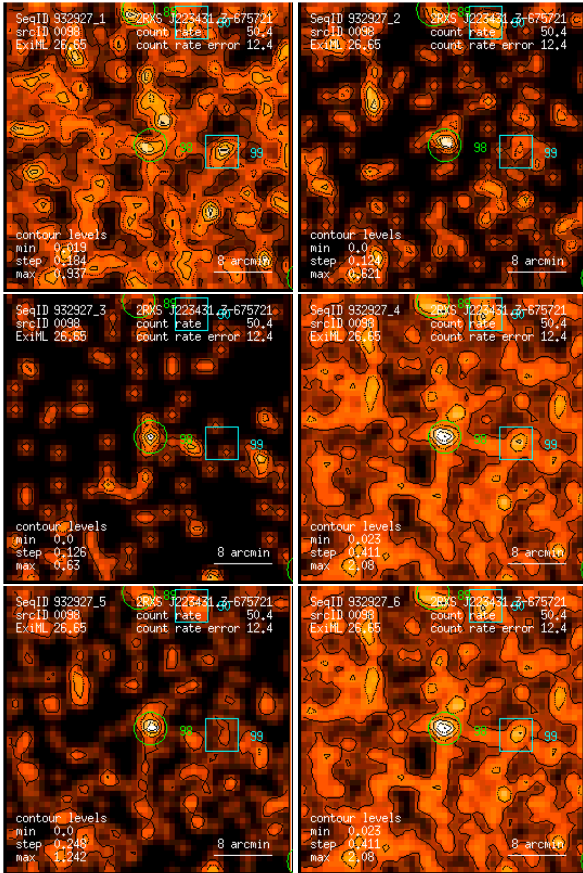
Figure 98: RASS 932927: detection 0098: band rate images, Gaussian filter: (1) PSPC channels 11 – 41, (2) 52 – 90, (3) 91 – 201, (4) 11 – 235, (5) 52 – 201, (6) 11 – 201. Broad band rates in counts/ks. Band rate contour levels in counts/ks/arcmin 2 .
