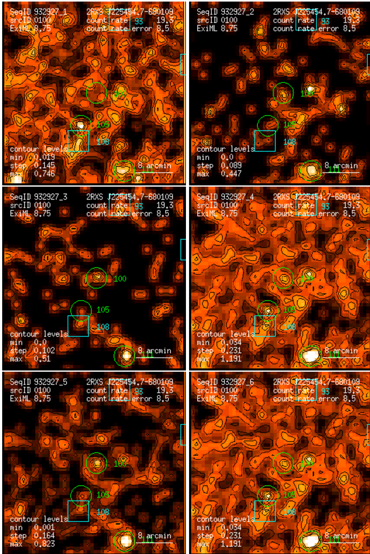
Figure 100: RASS 932927: detection 0100: band rate images, Gaussian filter: (1) PSPC channels 11 – 41, (2) 52 – 90, (3) 91 – 201, (4) 11 – 235, (5) 52 – 201, (6) 11 – 201. Broad band rates in counts/ks. Band rate contour levels in counts/ks/arcmin 2 .
