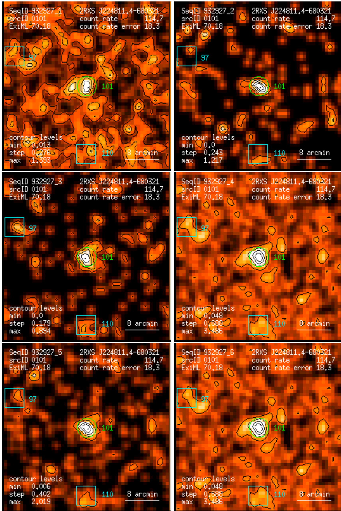
Figure 101: RASS 932927: detection 0101: band rate images, Gaussian filter: (1) PSPC channels 11 – 41, (2) 52 – 90, (3) 91 – 201, (4) 11 – 235, (5) 52 – 201, (6) 11 – 201. Broad band rates in counts/ks. Band rate contour levels in counts/ks/arcmin 2 .
