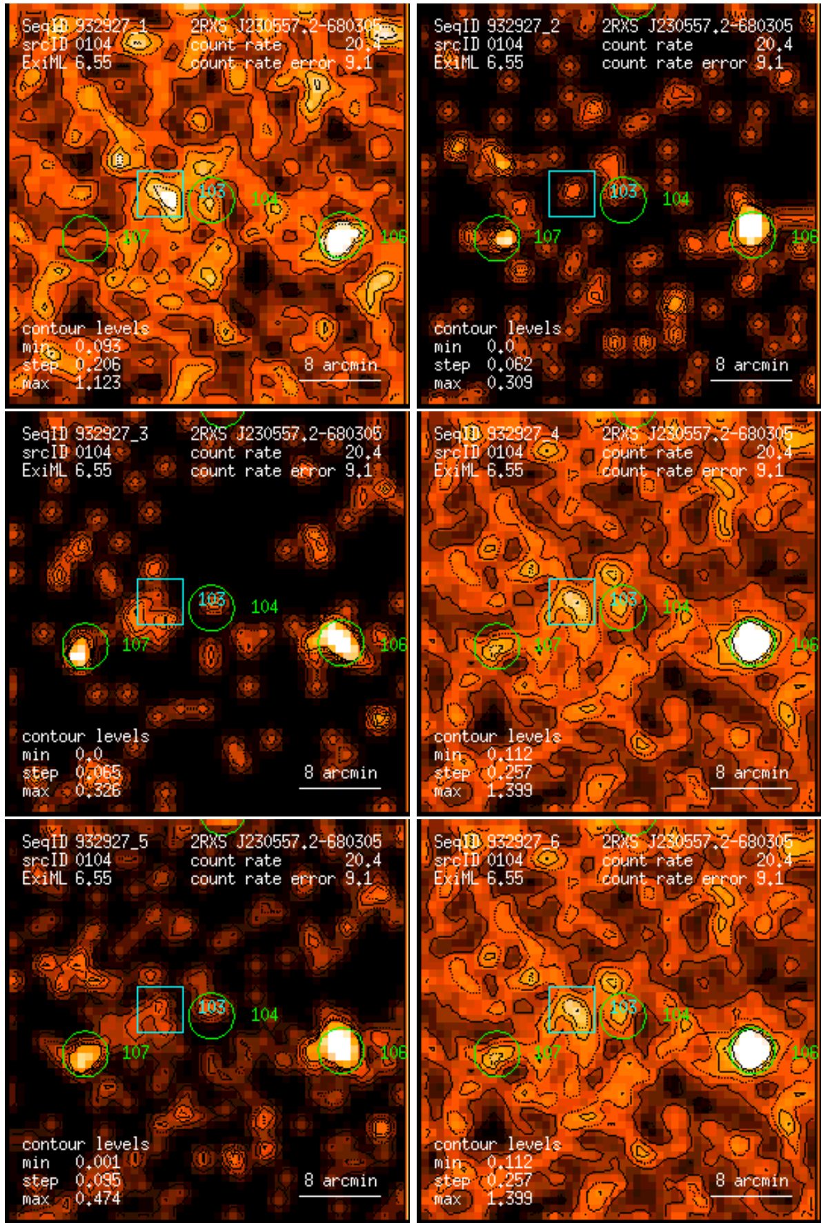
Figure 104: RASS 932927: detection 0104: band rate images, Gaussian filter: (1) PSPC channels 11 – 41, (2) 52 – 90, (3) 91 – 201, (4) 11 – 235, (5) 52 – 201, (6) 11 – 201. Broad band rates in counts/ks. Band rate contour levels in counts/ks/arcmin 2 .
