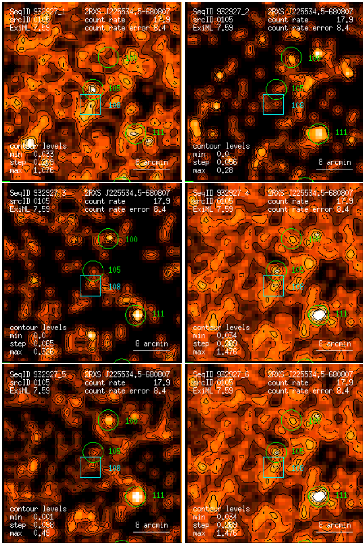
Figure 105: RASS 932927: detection 0105: band rate images, Gaussian filter: (1) PSPC channels 11 – 41, (2) 52 – 90, (3) 91 – 201, (4) 11 – 235, (5) 52 – 201, (6) 11 – 201. Broad band rates in counts/ks. Band rate contour levels in counts/ks/arcmin 2 .
