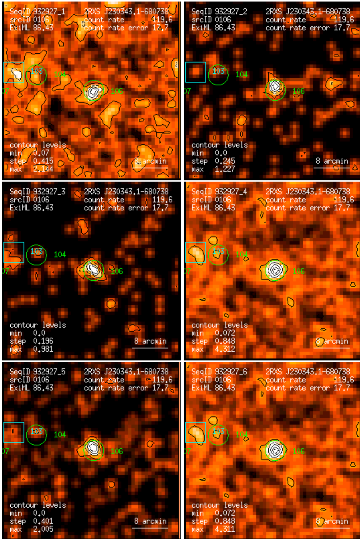
Figure 106: RASS 932927: detection 0106: band rate images, Gaussian filter: (1) PSPC channels 11 – 41, (2) 52 – 90, (3) 91 – 201, (4) 11 – 235, (5) 52 – 201, (6) 11 – 201. Broad band rates in counts/ks. Band rate contour levels in counts/ks/arcmin 2 .
