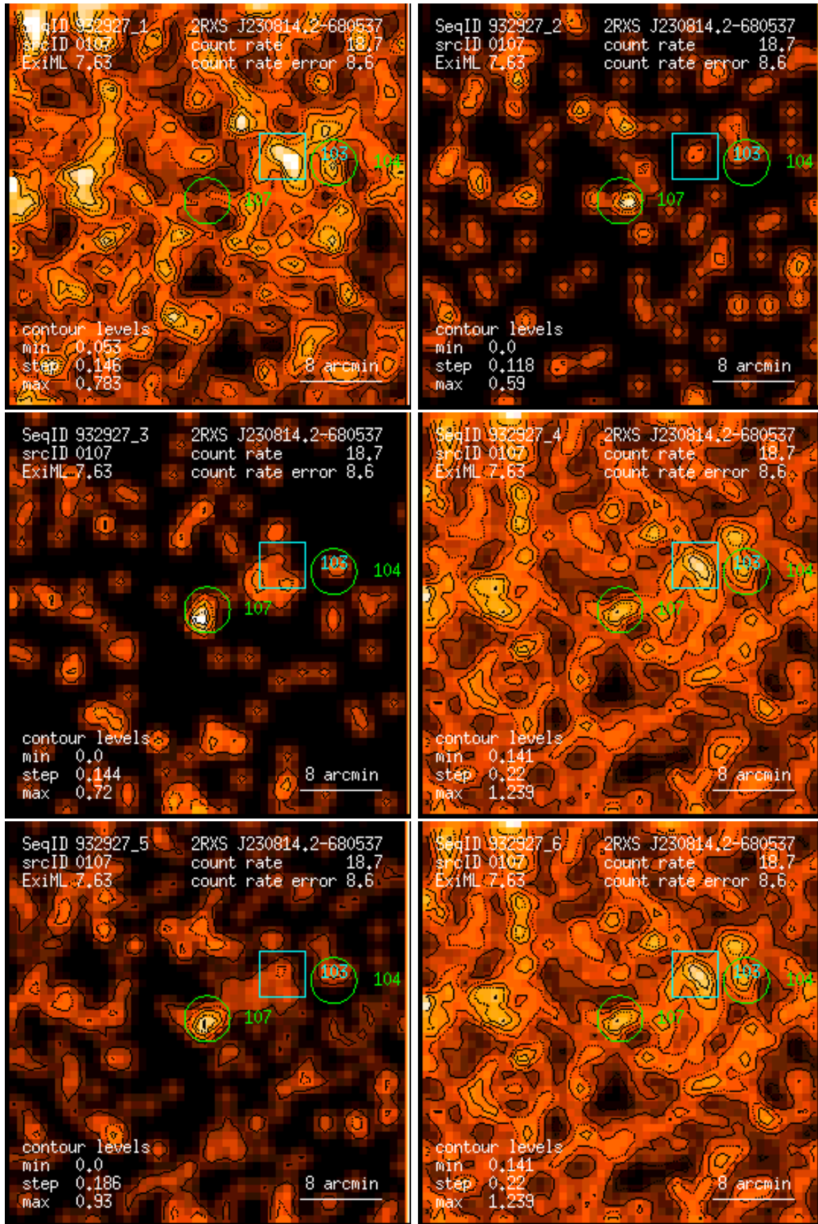
Figure 107: RASS 932927: detection 0107: band rate images, Gaussian filter: (1) PSPC channels 11 – 41, (2) 52 – 90, (3) 91 – 201, (4) 11 – 235, (5) 52 – 201, (6) 11 – 201. Broad band rates in counts/ks. Band rate contour levels in counts/ks/arcmin 2 .
