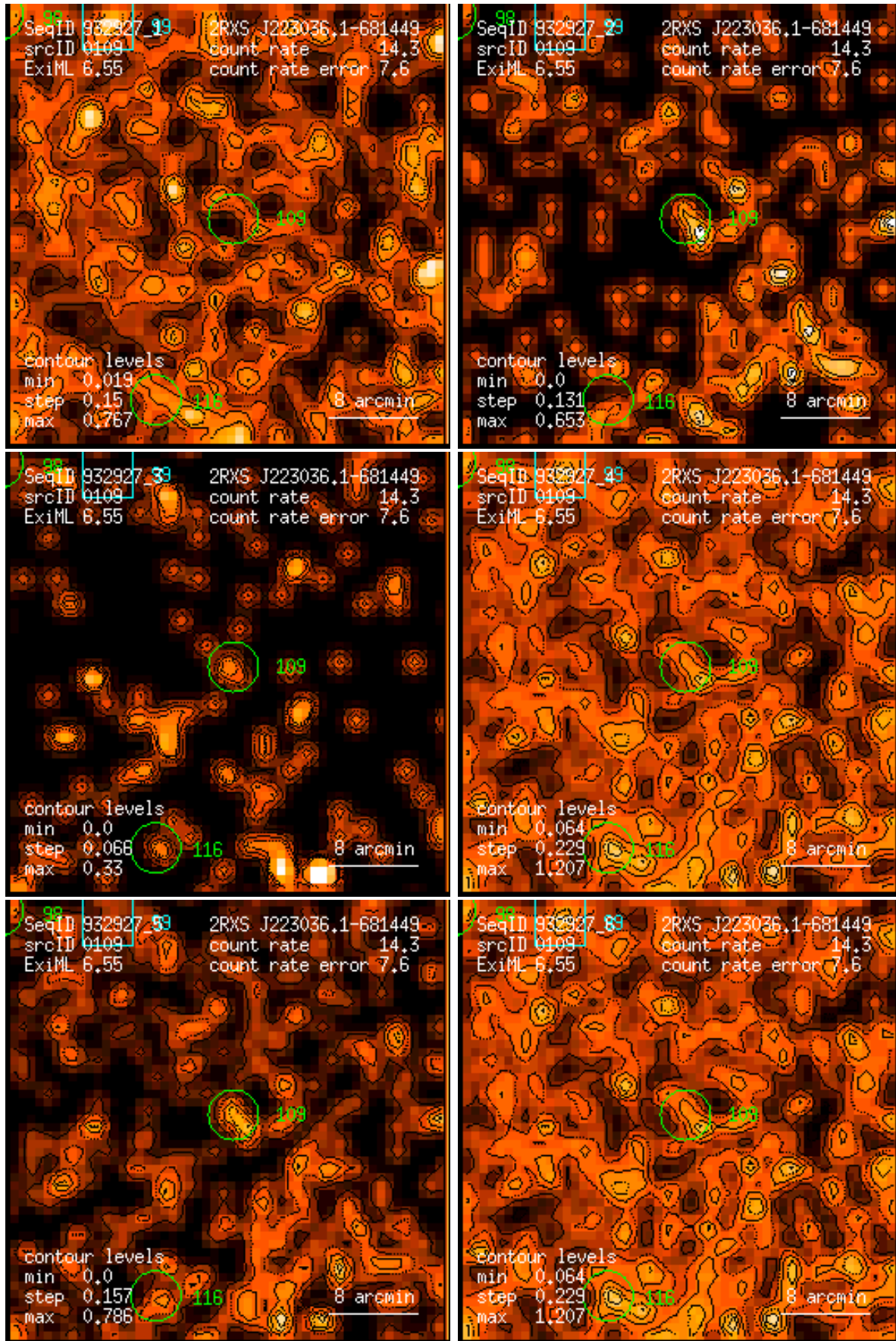
Figure 109: RASS 932927: detection 0109: band rate images, Gaussian filter: (1) PSPC channels 11 – 41, (2) 52 – 90, (3) 91 – 201, (4) 11 – 235, (5) 52 – 201, (6) 11 – 201. Broad band rates in counts/ks. Band rate contour levels in counts/ks/arcmin 2 .
