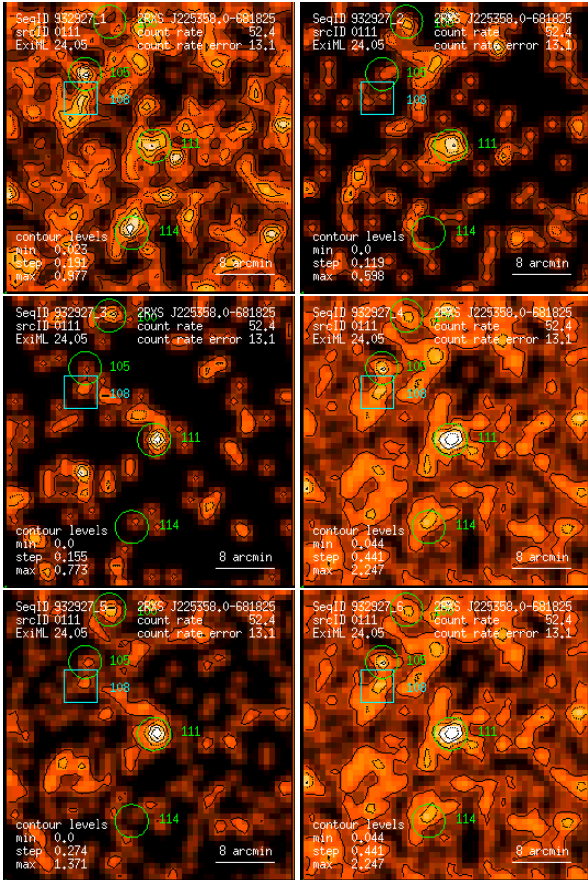
Figure 111: RASS 932927: detection 0111: band rate images, Gaussian filter: (1) PSPC channels 11 – 41, (2) 52 – 90, (3) 91 – 201, (4) 11 – 235, (5) 52 – 201, (6) 11 – 201. Broad band rates in counts/ks. Band rate contour levels in counts/ks/arcmin 2 .
