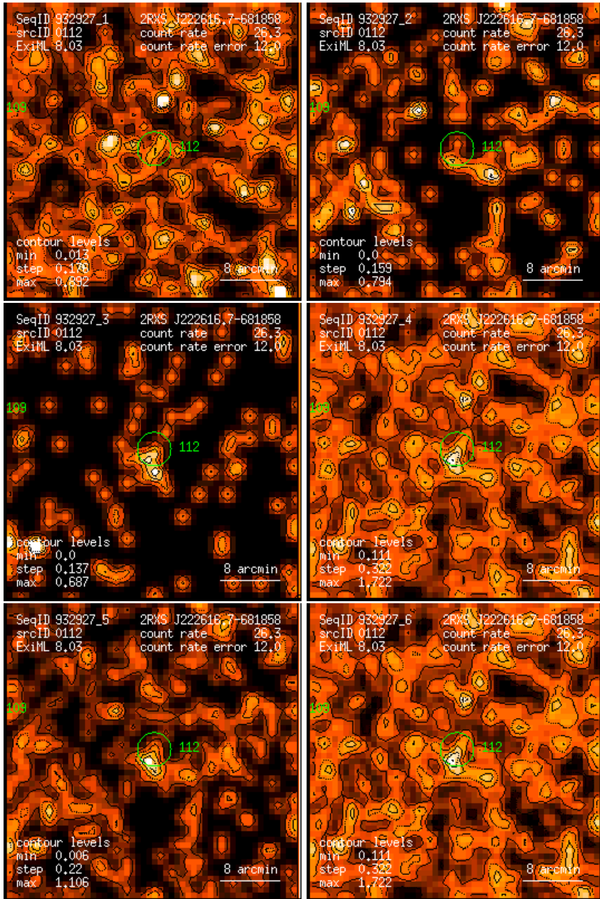
Figure 112: RASS 932927: detection 0112: band rate images, Gaussian filter: (1) PSPC channels 11 – 41, (2) 52 – 90, (3) 91 – 201, (4) 11 – 235, (5) 52 – 201, (6) 11 – 201. Broad band rates in counts/ks. Band rate contour levels in counts/ks/arcmin 2 .
