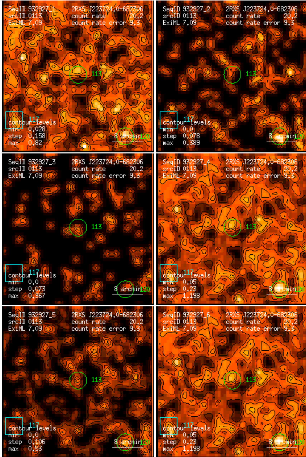
Figure 113: RASS 932927: detection 0113: band rate images, Gaussian filter: (1) PSPC channels 11 – 41, (2) 52 – 90, (3) 91 – 201, (4) 11 – 235, (5) 52 – 201, (6) 11 – 201. Broad band rates in counts/ks. Band rate contour levels in counts/ks/arcmin 2 .
