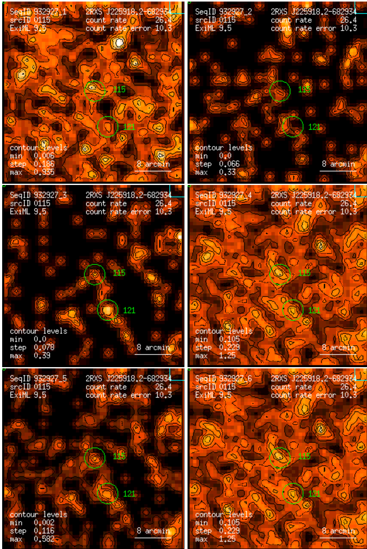
Figure 115: RASS 932927: detection 0115: band rate images, Gaussian filter: (1) PSPC channels 11 – 41, (2) 52 – 90, (3) 91 – 201, (4) 11 – 235, (5) 52 – 201, (6) 11 – 201. Broad band rates in counts/ks. Band rate contour levels in counts/ks/arcmin 2 .
