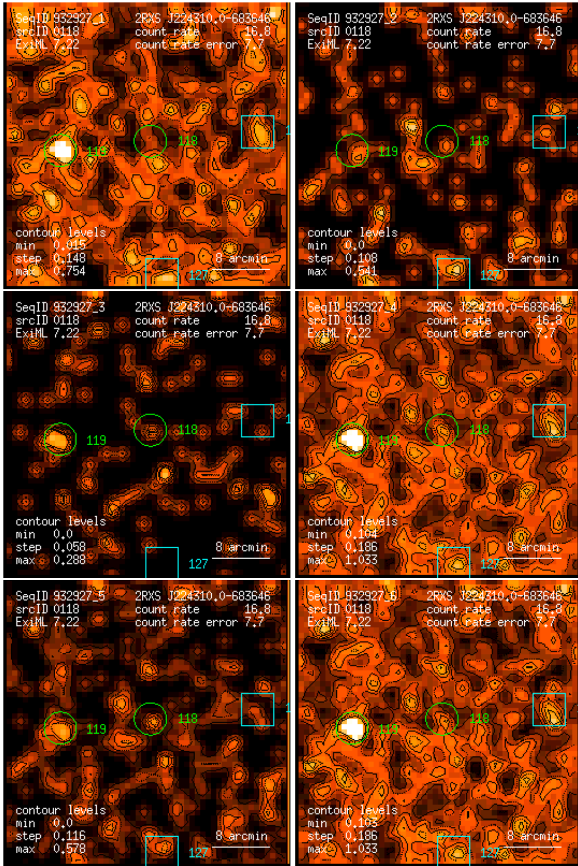
Figure 118: RASS 932927: detection 0118: band rate images, Gaussian filter: (1) PSPC channels 11 – 41, (2) 52 – 90, (3) 91 – 201, (4) 11 – 235, (5) 52 – 201, (6) 11 – 201. Broad band rates in counts/ks. Band rate contour levels in counts/ks/arcmin 2 .
