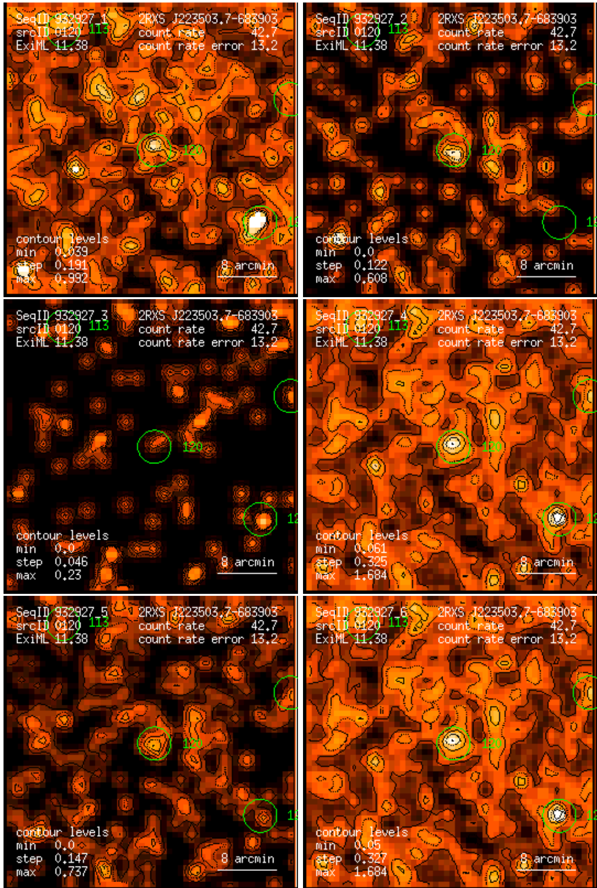
Figure 120: RASS 932927: detection 0120: band rate images, Gaussian filter: (1) PSPC channels 11 – 41, (2) 52 – 90, (3) 91 – 201, (4) 11 – 235, (5) 52 – 201, (6) 11 – 201. Broad band rates in counts/ks. Band rate contour levels in counts/ks/arcmin 2 .
